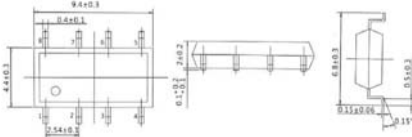
Dimensions外形尺寸
