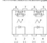
Terminal Identification 引脚标识
