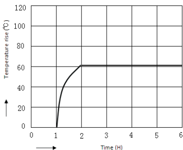
Coil temperature rise (ambient temperature 23 °C)
